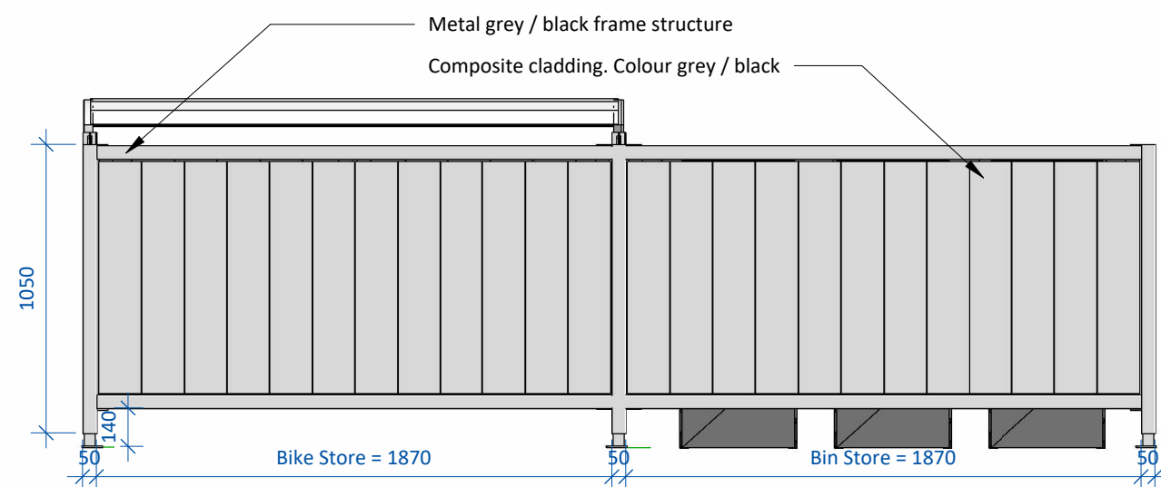
Rear Elevation; 1:25
