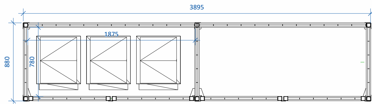
Section Plan; 1:25
