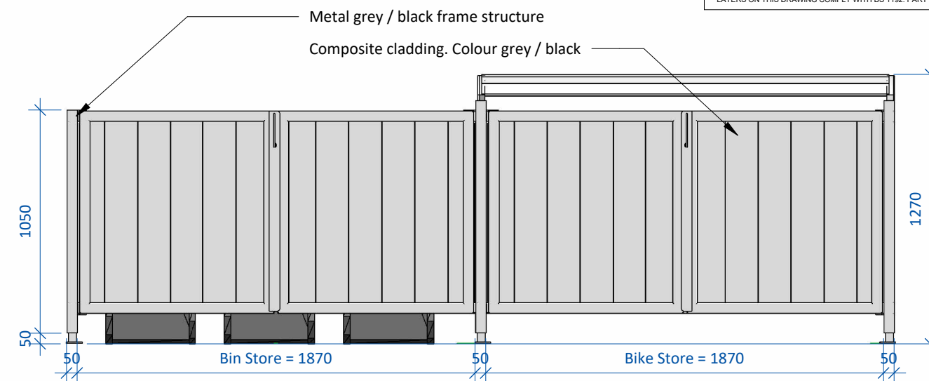
Front Elevation; 1:25
