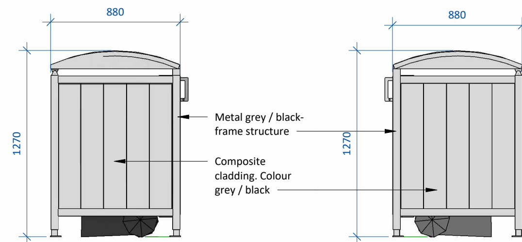
Side Elevation 1; 1:25
