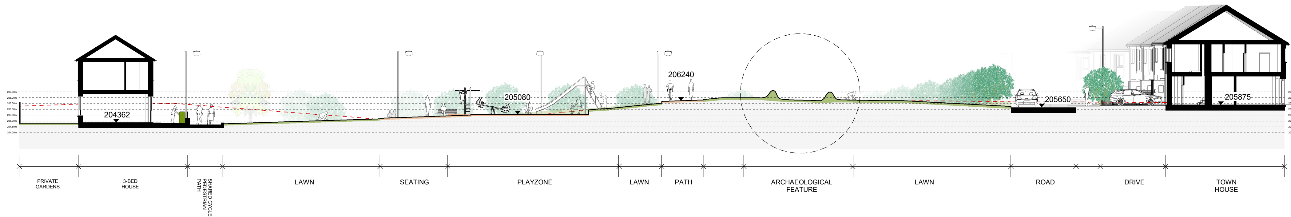
SECTION A-A THROUGH MAIN PUBLIC OPEN SPACE
